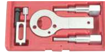
■ 920G2 P.1-12 Engine timing Tool set for Opel / Vauxhall
