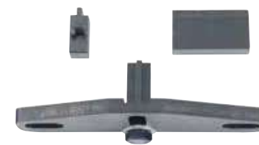
■ 9G1211 P.1-18 Camshaft setting bar & TDC timing pins (Ford / Mazda)
